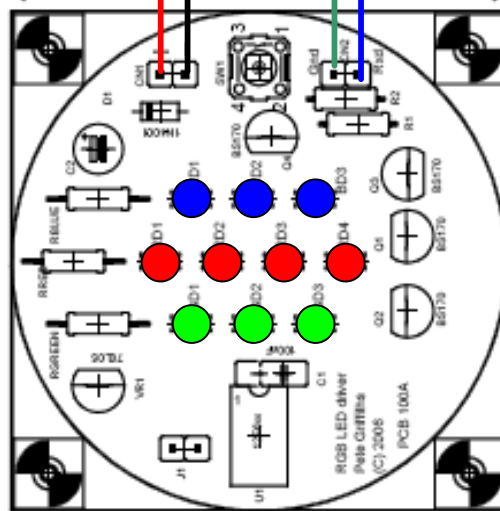
Simple RGB LED Driver Board
