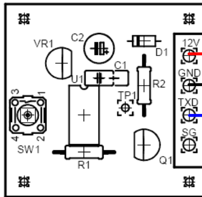
Simple RGB Controller Board
