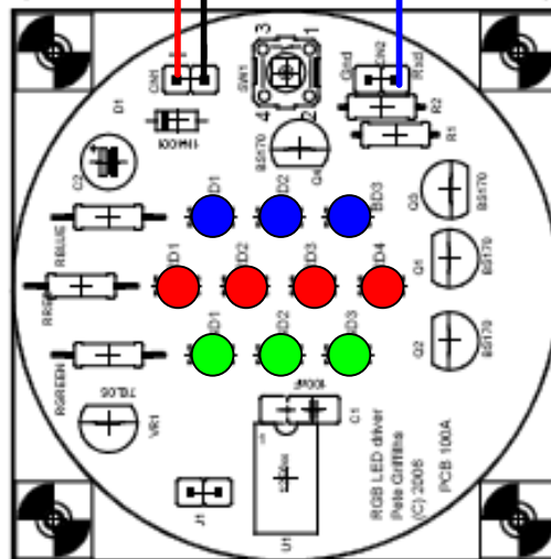
Simple RGB LED Driver Board
