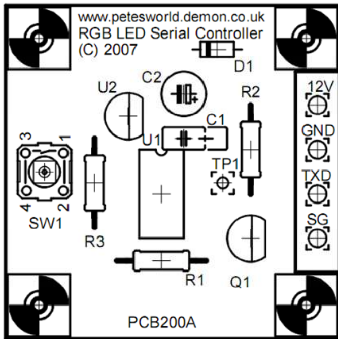
Simple RGB Controller Board
